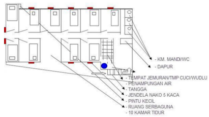
DENAH LANTAI 2
